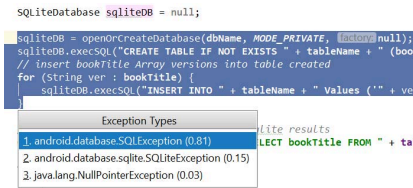
Figure 2: Recommendation for the usage of object SQLiteDatabase
